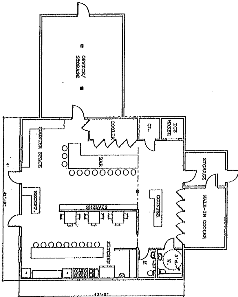
FLOOR PLAN SCALE: 3/16"=1'-0"
